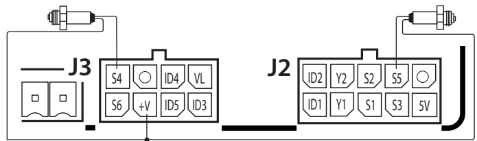
4-20 mA probes
